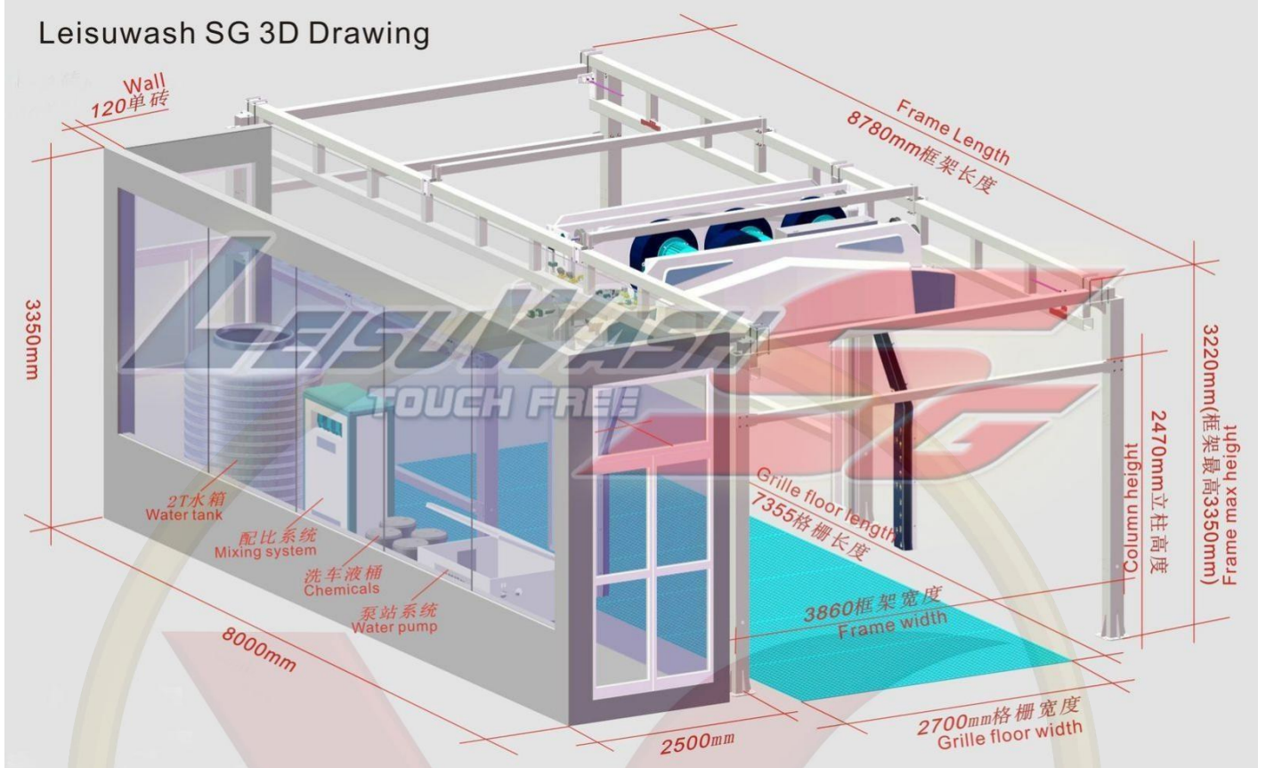
Leisuwash SG Car Wash Equipment 3D Drawing
